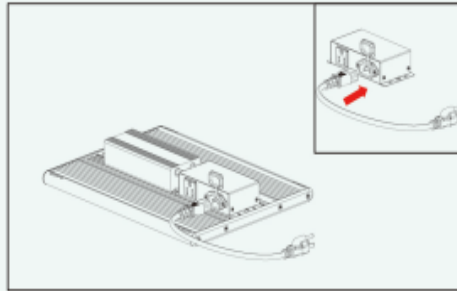
4 . Connect the controller with AC cable
