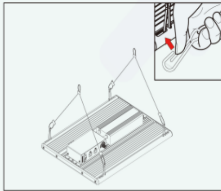
1 . hang up 4-foot steel hanger
