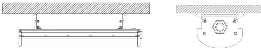
Ceiling Mounting
