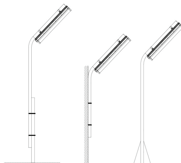
Pole Mounting
